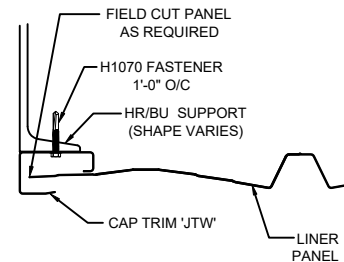
SECTION 'L120' w/ HR/BU SUPPORT
