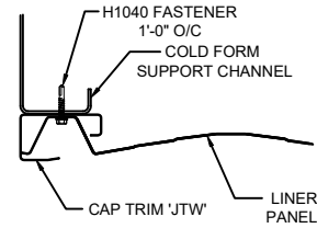
SECTION 'L120' w/ COLD FORM CHANNEL AND ALTERNATE PANEL FINISH
