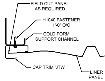
SECTION 'L120' w/ COLD FORM CHANNEL
