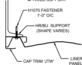
SECTION 'L120' w/ HR/BU SUPPORT AND ALTERNATE PANEL FINISH
