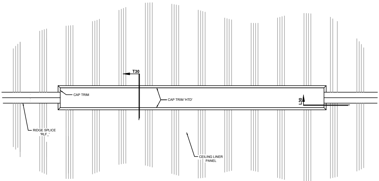
IF0030 CEILING LINER AT PEAK w/ RIDGE VENTS
