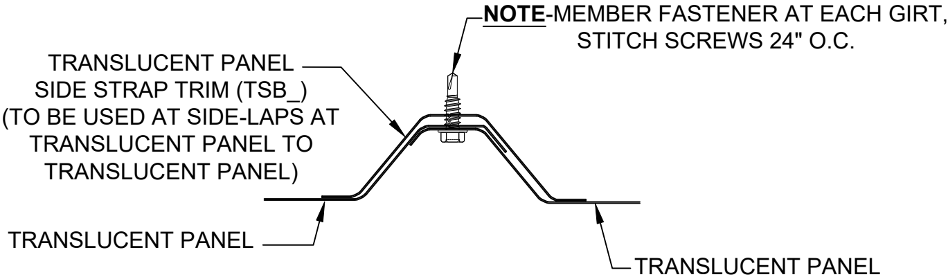
DETAIL "A"
