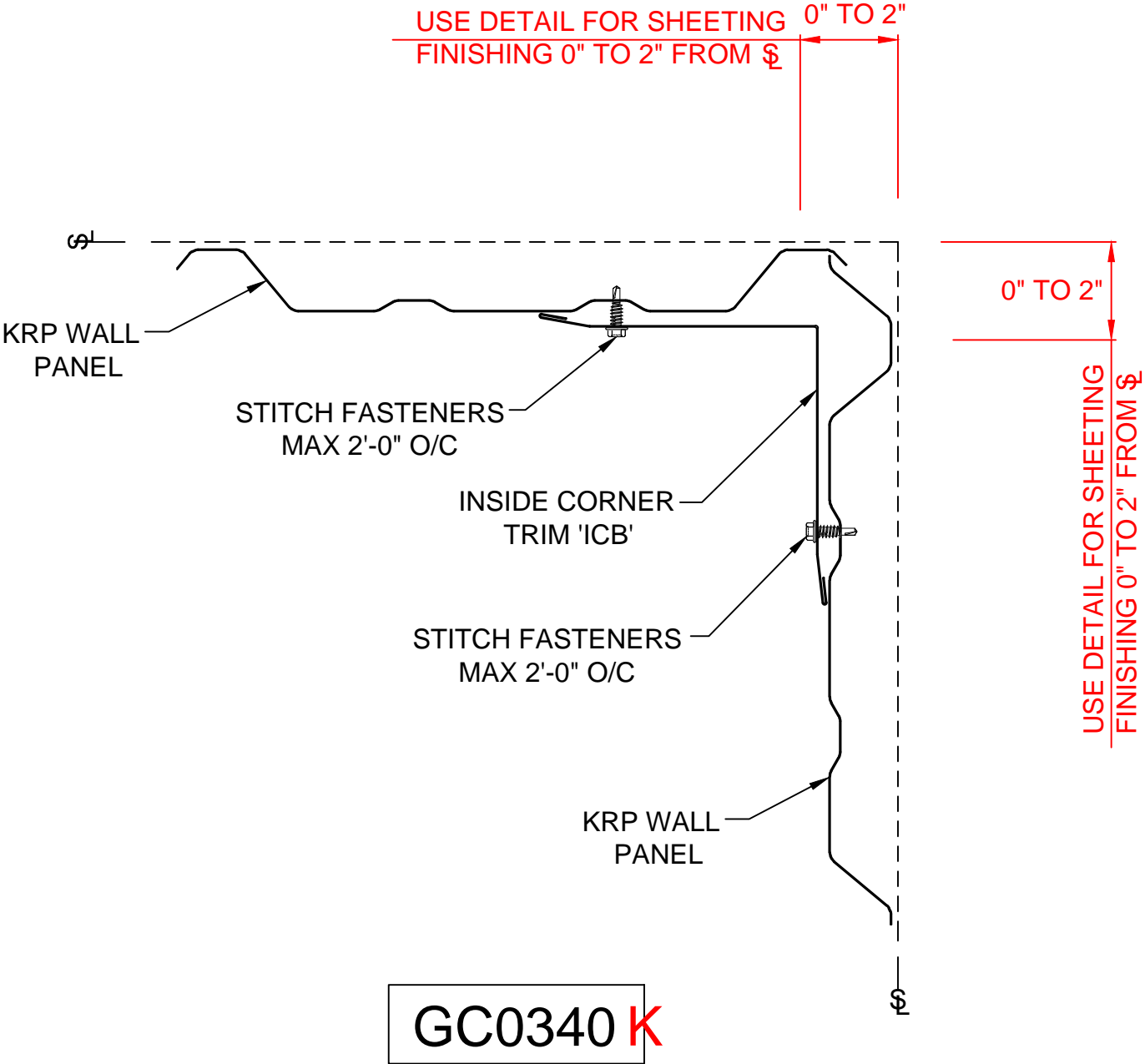
KRP PANEL INSIDE CORNER DETAIL
