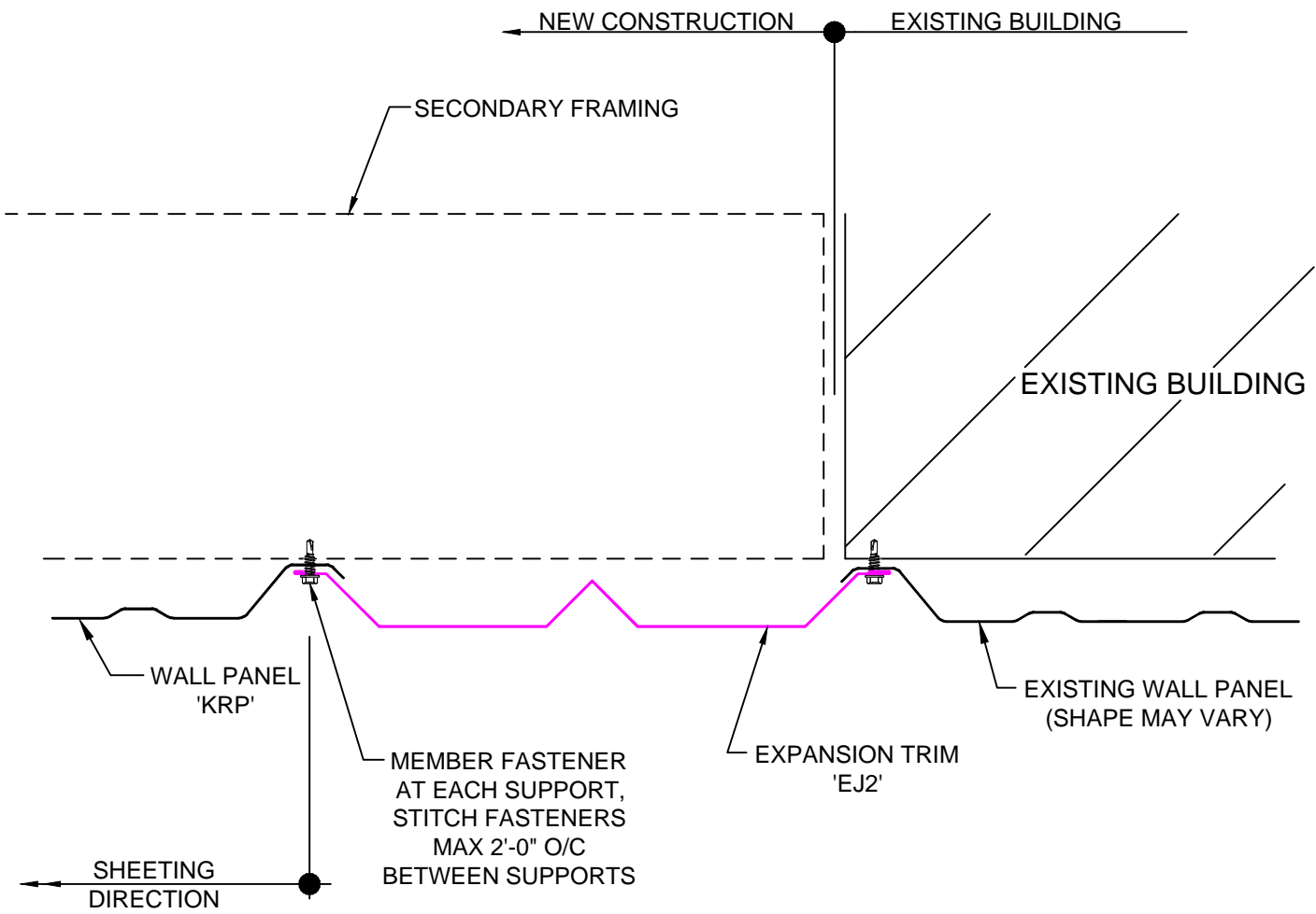
GC0364 K KRP PANEL TIE-IN TO EXISTING PANEL w/ TRIM
