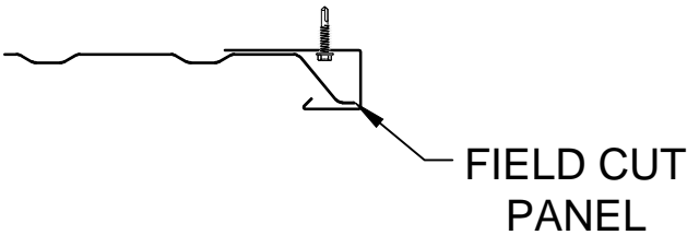
ALTERNATE FINISH DETAIL
