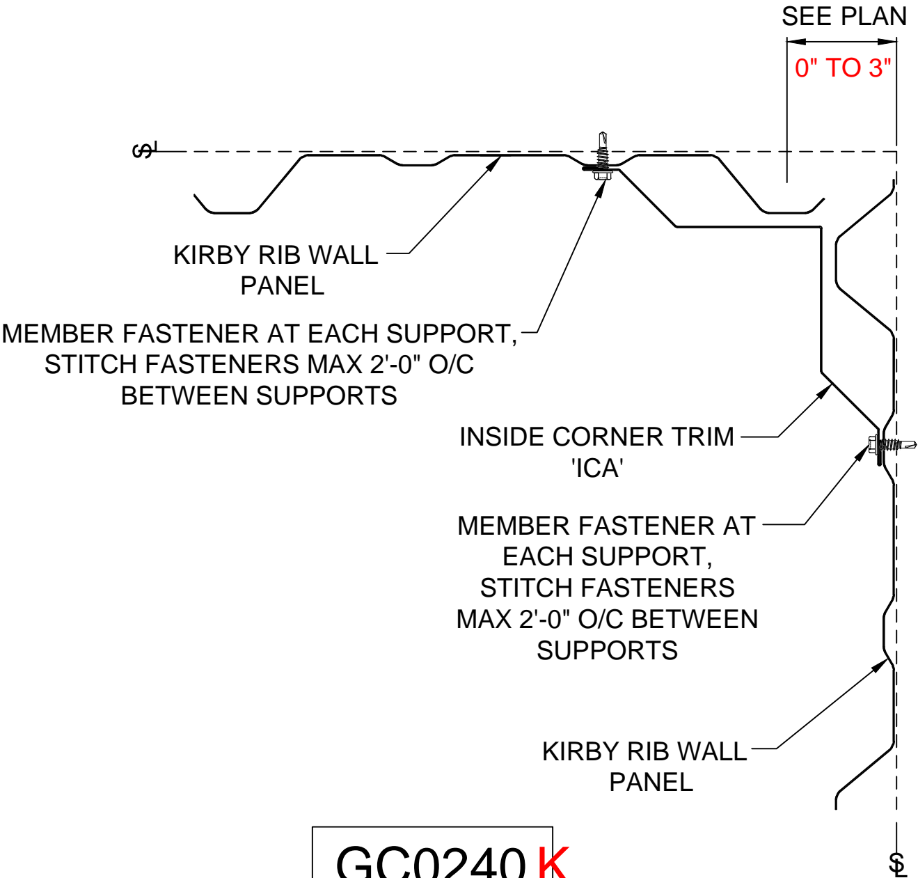
KIRBY RIB PANEL INSIDE CORNER DETAIL
