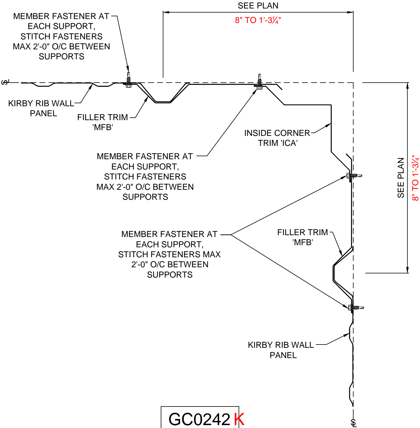
KIRBY RIB PANEL INSIDE CORNER DETAIL W/ FILLER TRIM BOTH SIDES
