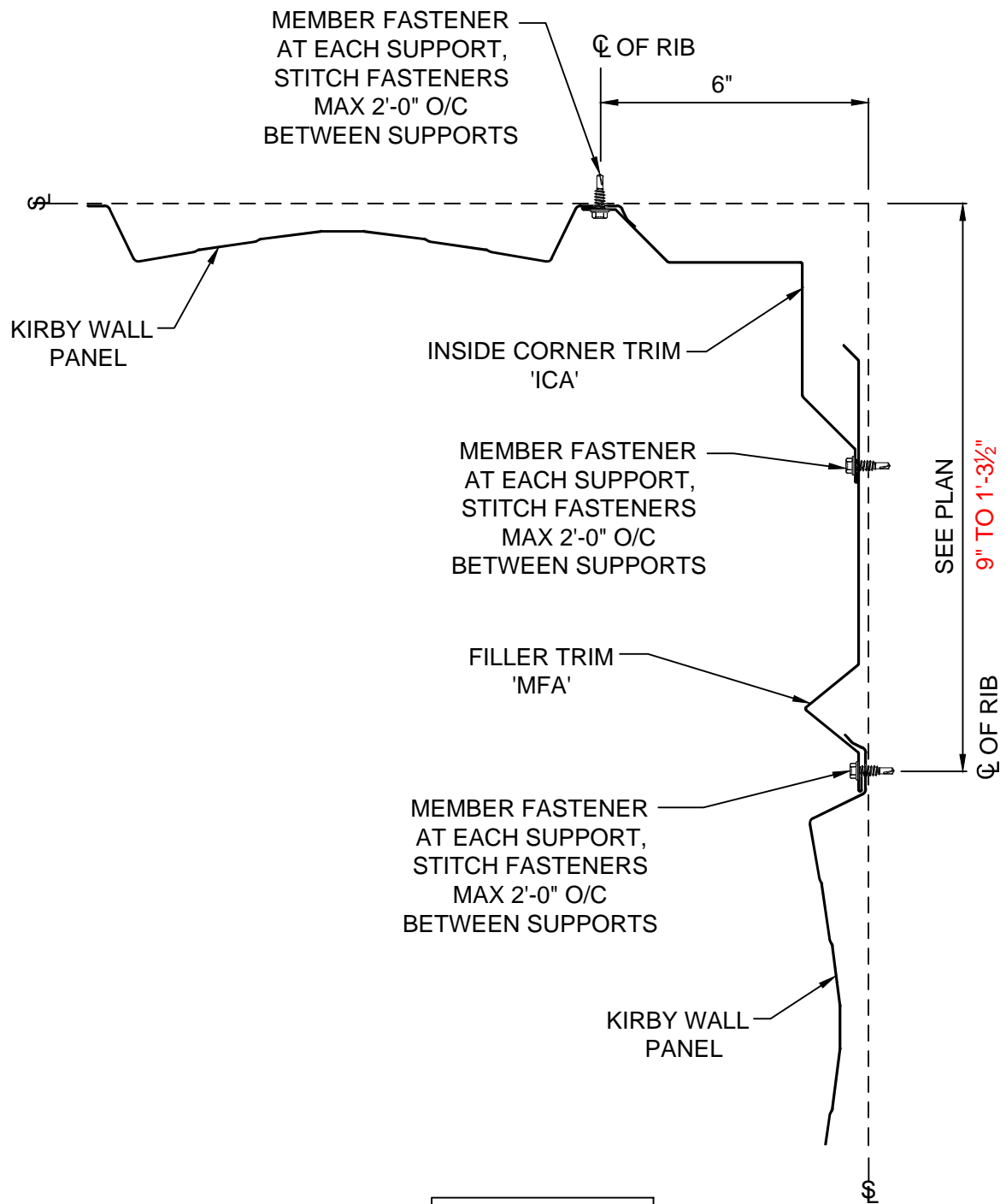
KIRBY WALL PANEL INSIDE CORNER DETAIL W/ FILLER TRIM ONE SIDE
