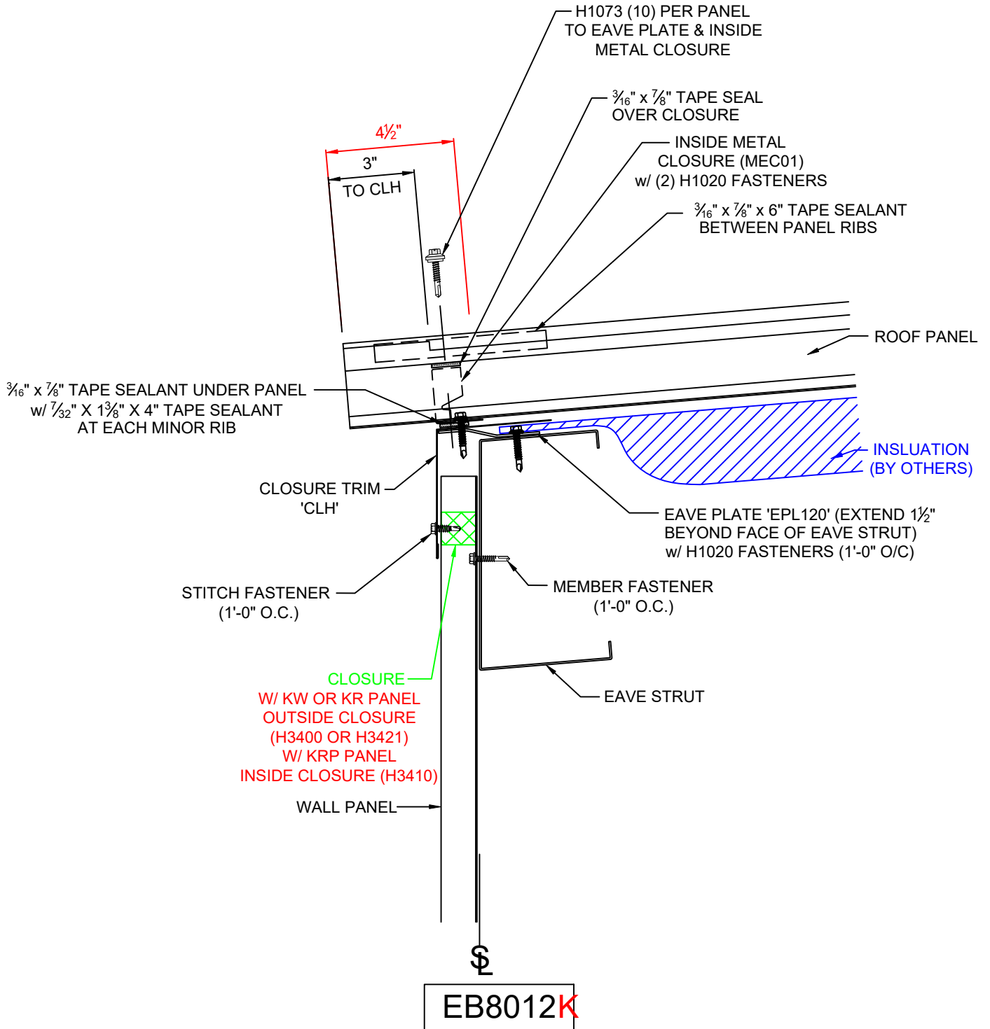
SS360 LOW SYSTEM EAVE w/ SIMPLE EAVE FLASH & SHEETED WALL w/ FIRST PURLIN < 3'-0" UPHILL
