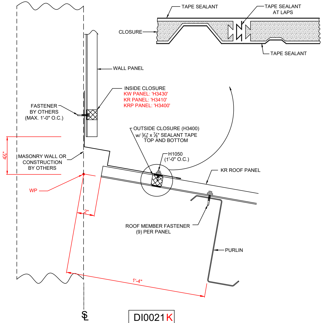
KIRBYRIB ROOF TO WALL DETAIL, PANEL ABOVE ON FRAMING BY OTHERS
