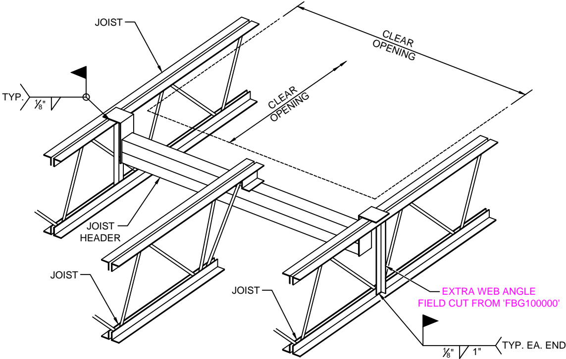
ISOMETRIC VIEW
