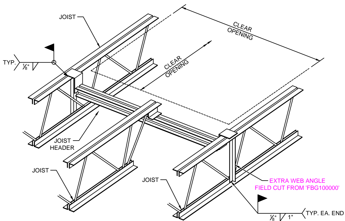
ISOMETRIC VIEW
