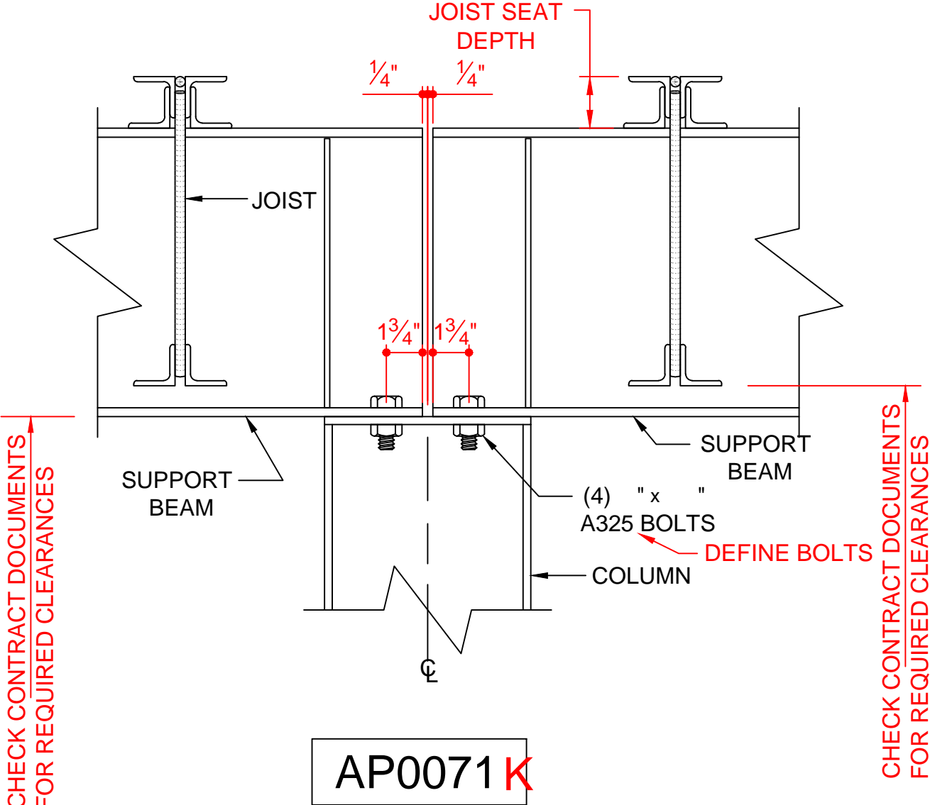
MEZZANINE BEAMS TO INTERIOR "I" SHAPE COLUMN
